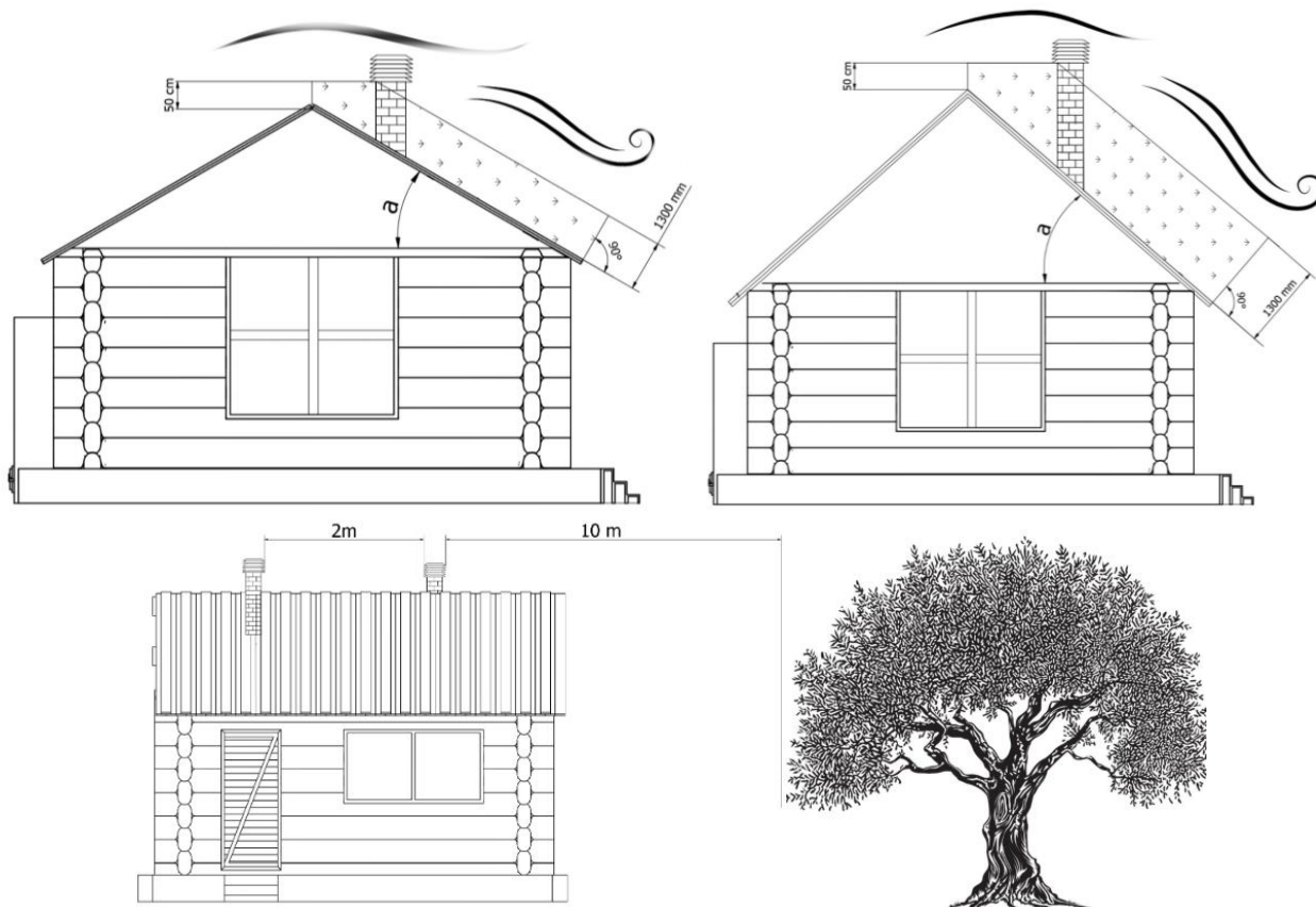
Figure 3 - Chimney – Positioning and distance
