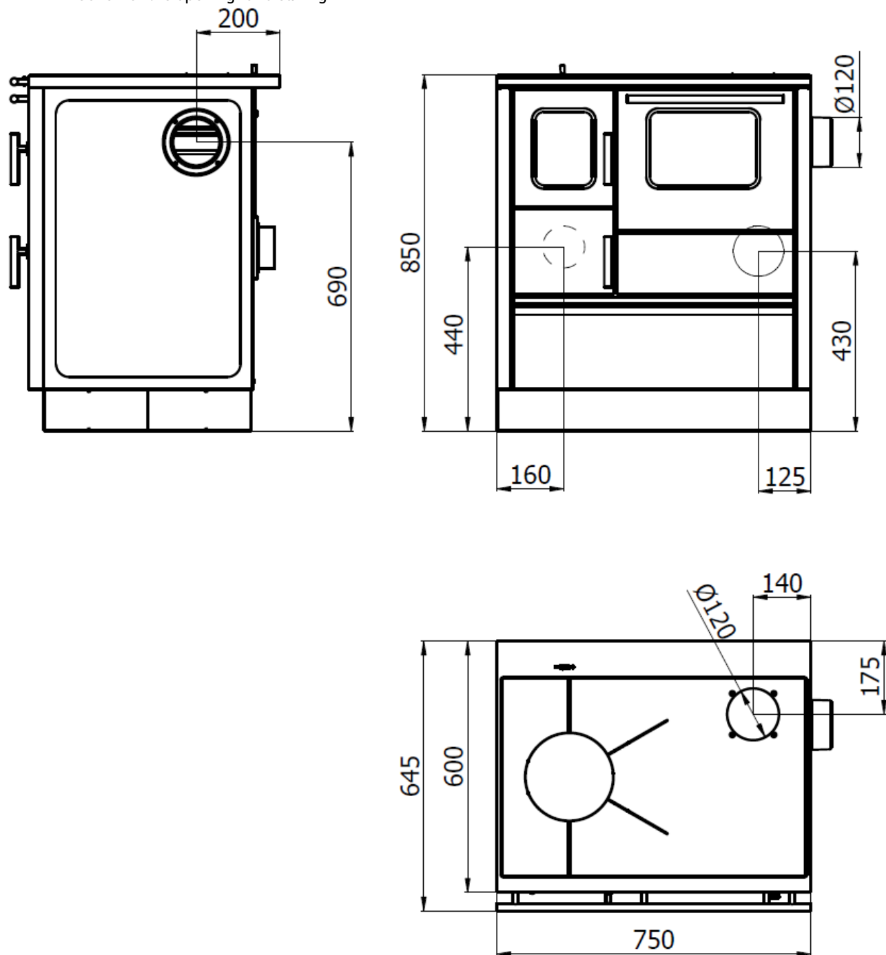
Figure 2 - Inox 75- Dimensions
